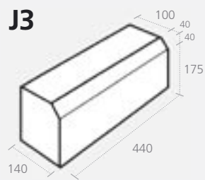
Chamfered Plinth
