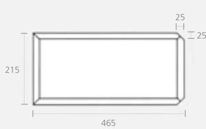
Chamfered Quoin
