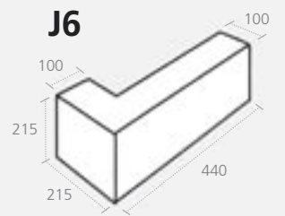
Plain Quoin
