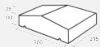
Keystone
