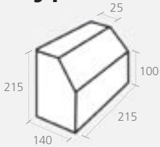
Coping Blocks
