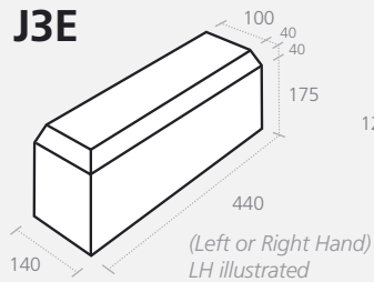
Chamfered Plinth External Return
