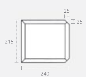
Plain Quoin
